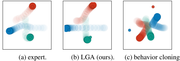
Figure 3: Example trajectories generated by (a) expert, (b) LGA, and (c) behavior cloning.
